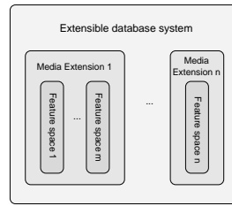
Fig. 1 An extensible DBMS architecture with multimedia extensions
