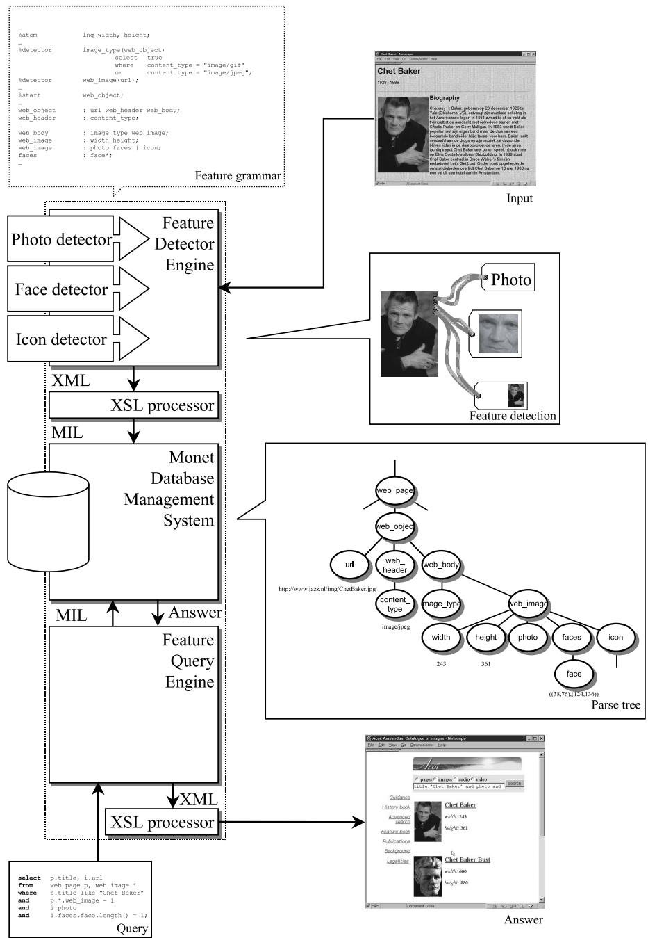
Fig. 5 Acoi architecture
