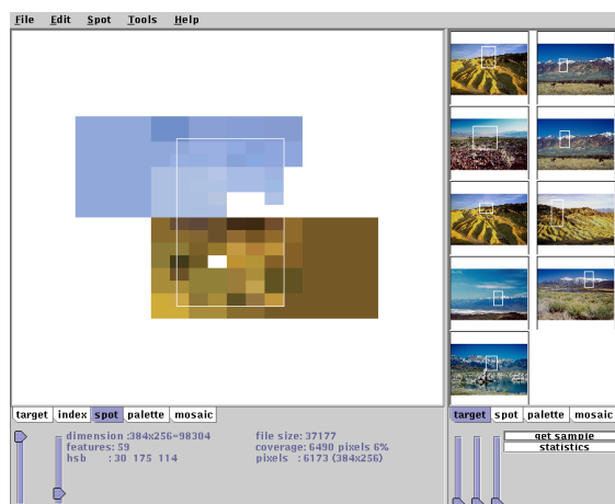
Fig. 3 A user interface supporting spot-based retrieval
